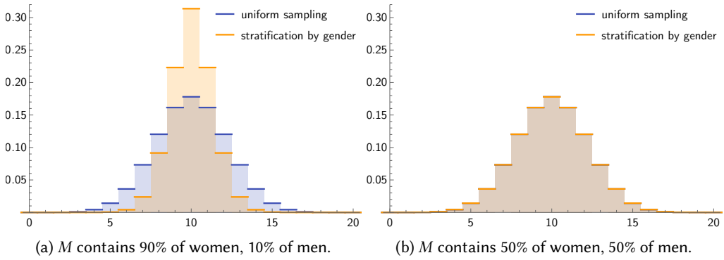
Fig. 1. Probabilities of different numbers of agents from M in the panel. The population consists of 500 women and 500 men; the panel has size 20; 500 agents are in M , distributed among genders as indicated.
