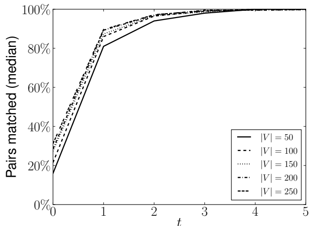
Figure 4: Pairs matched (% , y-axis) in generated UNOS graphs of varying sizes (lines), as t increases (x-axis).
