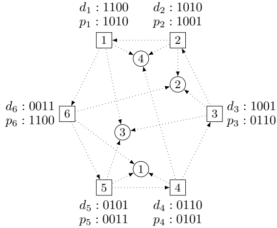
Figure 1: Gadget G_4 with a subset of non -edges shown; all edges between circle vertices are also not in E .
