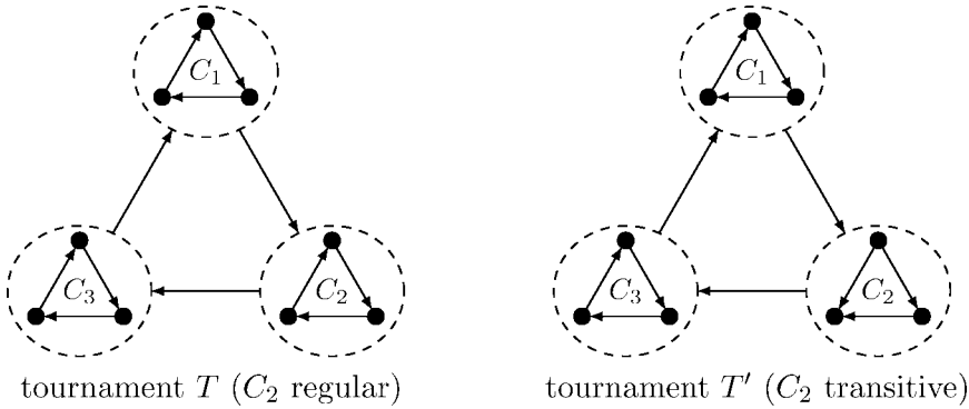
Fig. 1. Tournaments used in the proof of Theorem 3.2, illustrated for k = 3 . A voting tree is assumed to select an alternative from C_1 .
