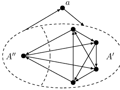
Fig. 2. Tournament structure providing an upper bound for the randomized k -caterpillar, example for m = 6 and \epsilon = 1/5 . A' and A'' contain (1 - \epsilon)(m - 1) and \epsilon(m - 1) alternatives, respectively.
