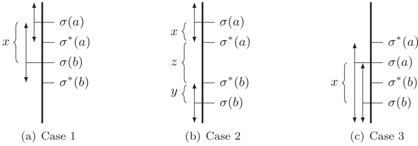
Fig. 1. Exchanges under the footrule and the maximum displacement distances.
