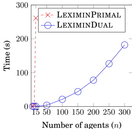
Fig. 1. Running time of LEXIMINPRIMAL and LEXIMINDUAL.
